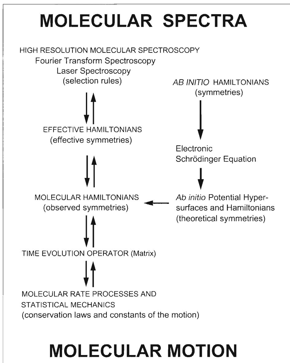
Fig. 1. Scheme to derive fundamental processes of molecular kinetics from high-resolution spectroscopy (after [12])
