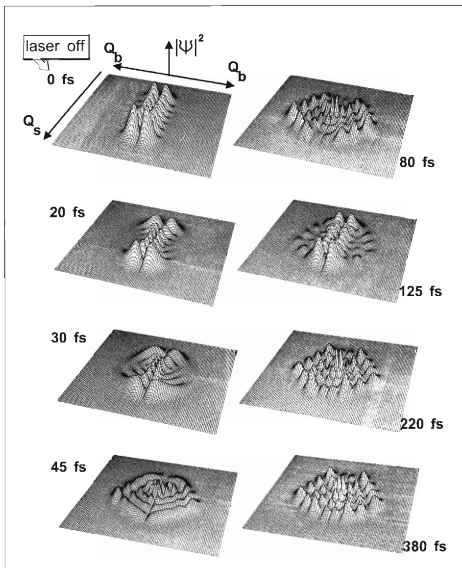
Fig. 4. Wavepacket motion for the two strongly coupled CH-stretching ( Q_s ) and CH-bending ( Q_b ) vibrations in the \text{CHF}_3 molecule |\Psi(Q_s, Q_b, t)|^2 is the probability distribution on the fs time scale after initial CH-stretching excitation at t = 0 (after [11])
